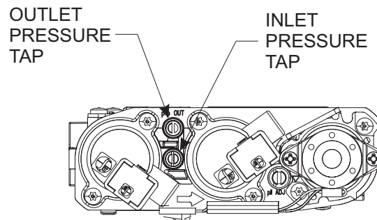
Figure 6 - IP Valve
