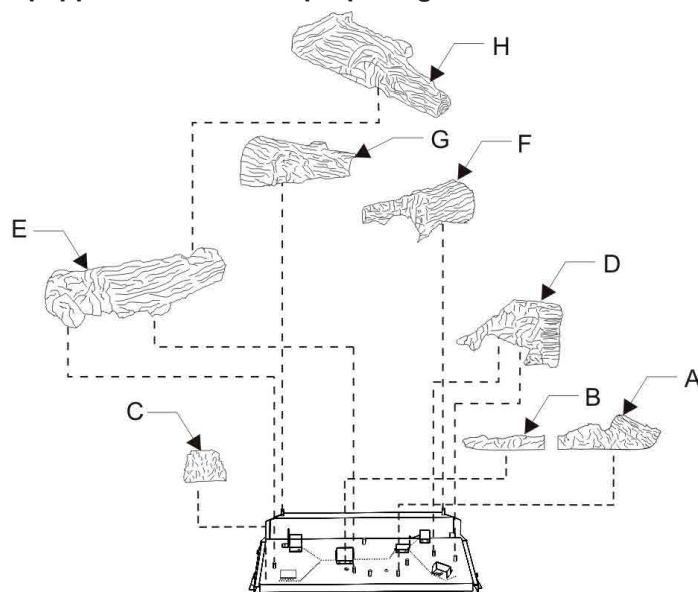
Log Placement - OLX(24,30)WR-1 Logs
