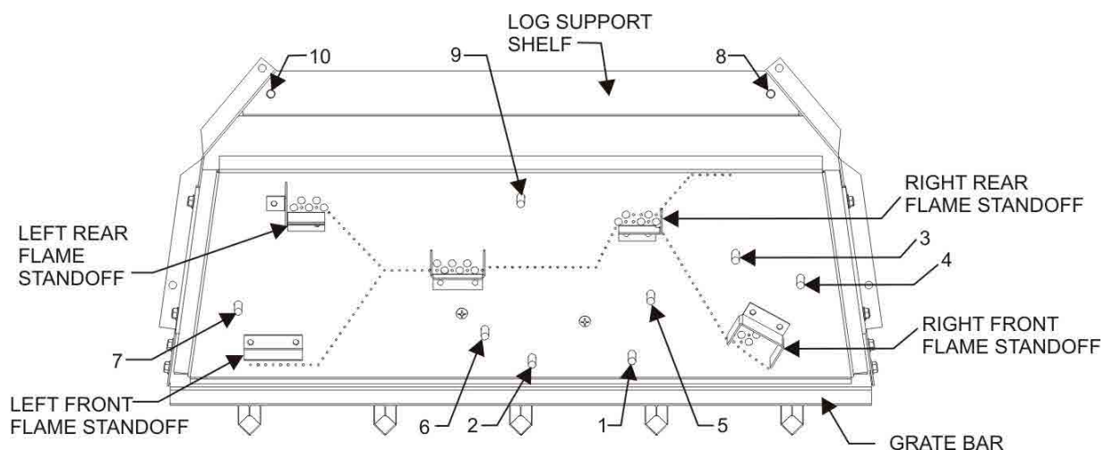
Burner Pin Location
