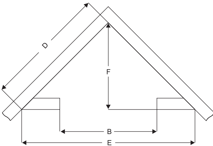
Rough Opening for Installing in Corner
