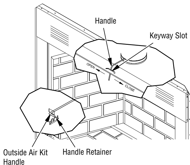
Figure 22 - Damper and Air Kit Handle
