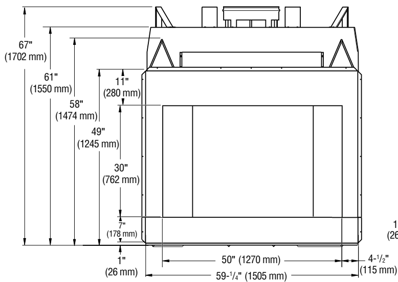
Figure 3 - 50" Model WRT6050
