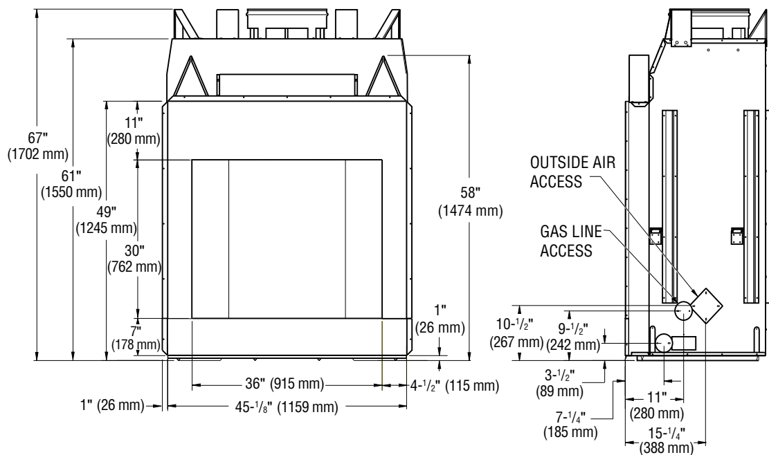
Figure 1 - 36" Model WRT6036
