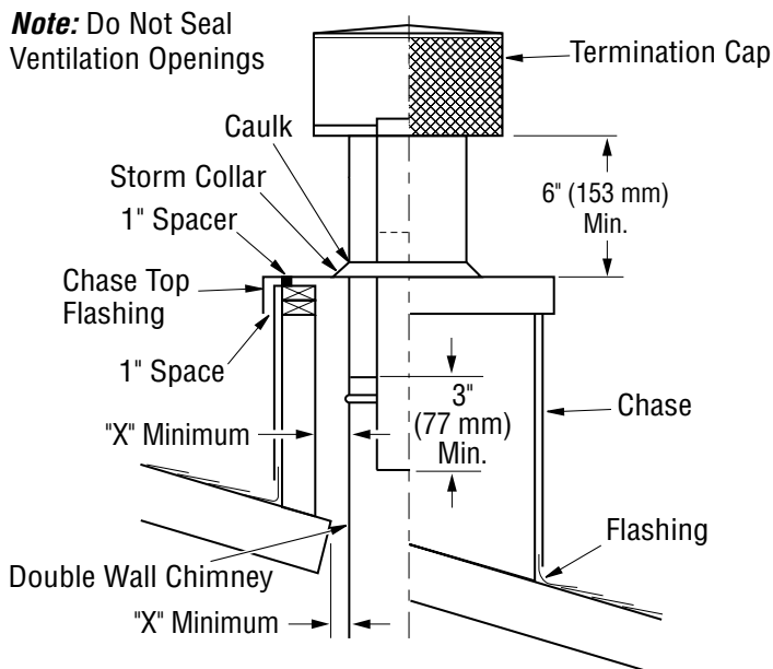
Figure 29 - Chase Installation
