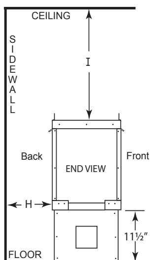
Figure 11 - See-through fireplace clearance to combustibles (See Table 5)
