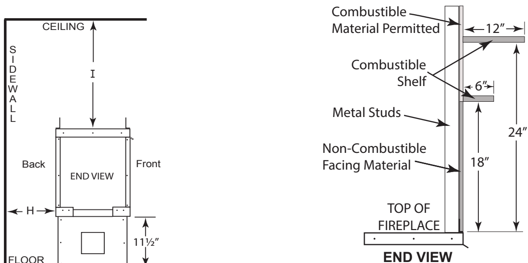
Figure 6 - Single-sided fireplace clearance to combustibles (See Table 3)
