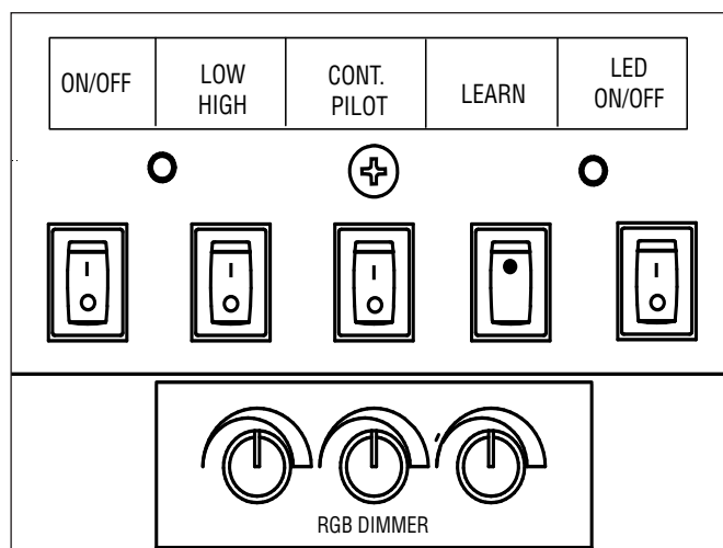
Figure 43 - Control panel
