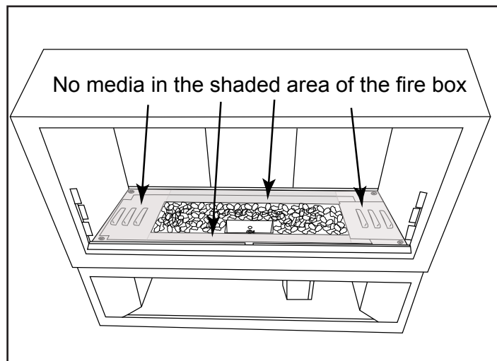
Figure 37 Covering the entire fireplace floor is NOT permitted in the shaded area.
