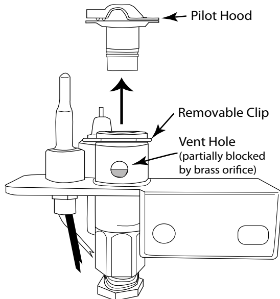
Figure 50 - Pilot Hood Removal
