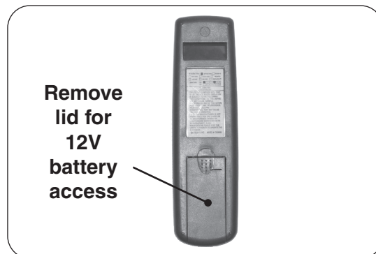
Fig. 45-2 Transmitter battery
