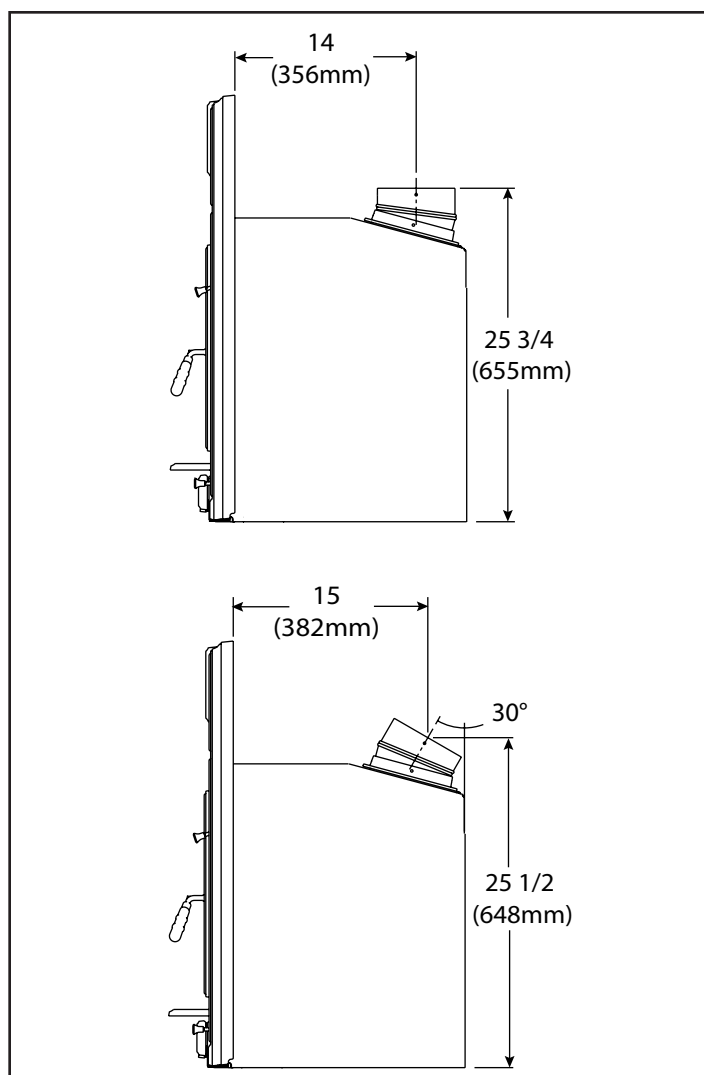
Figure 7.3 - Side View With Optional Offset Adapter
