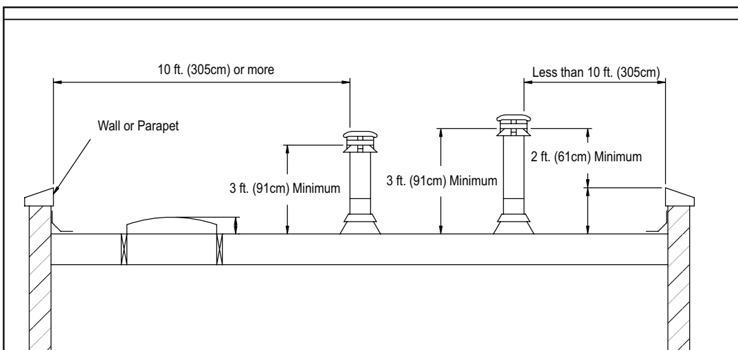
Figure 11.2 Flat Roof
