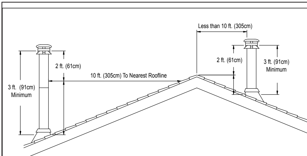
Figure 11.1 Pitched Roof
