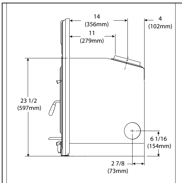
Figure 7.4 - Side View
