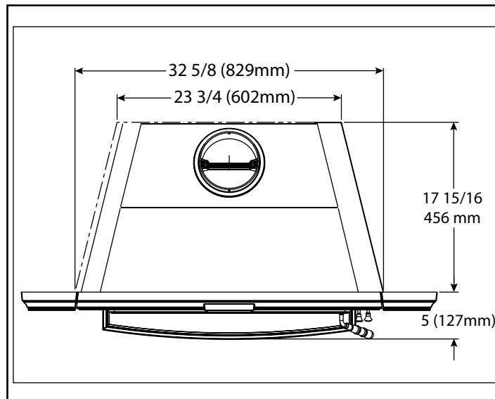
Figure 7.2 Top View
