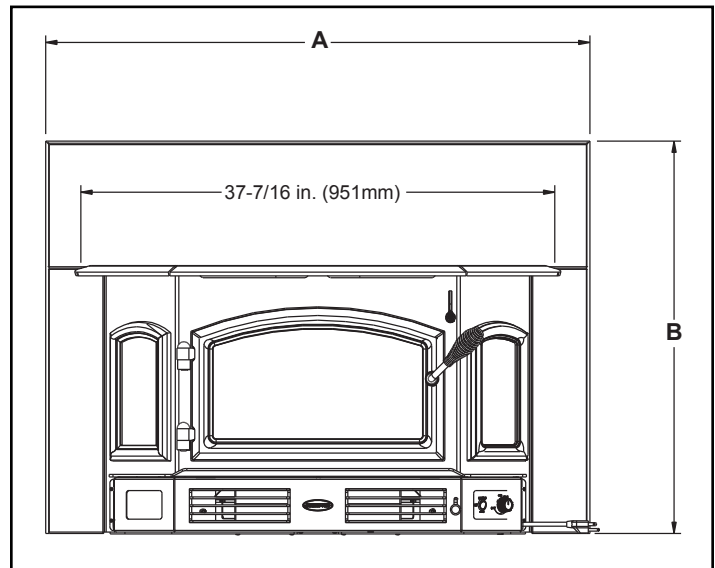
Figure 7.2 Front View
