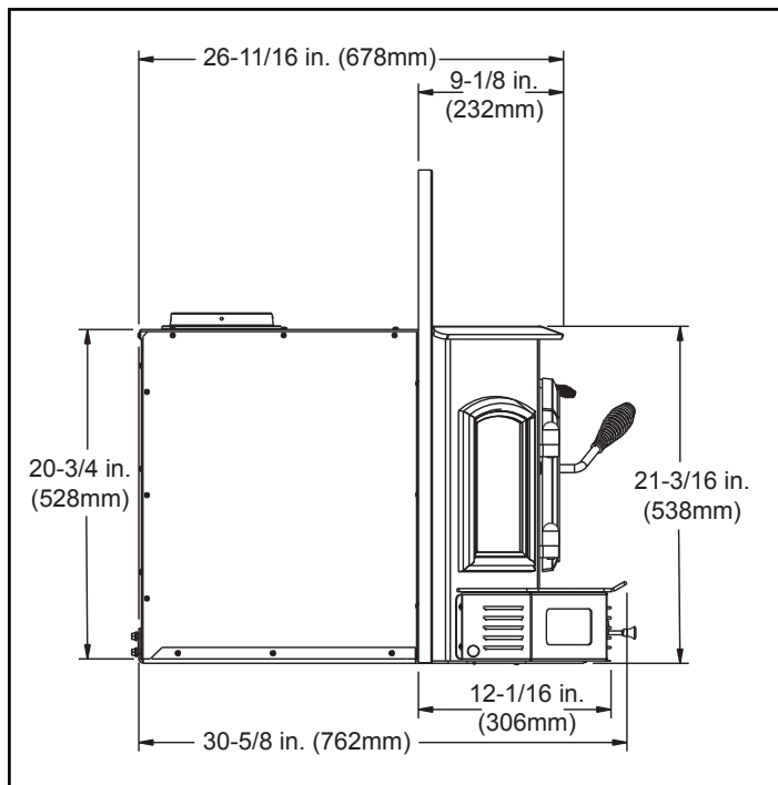
Figure 7.3 - Side View
