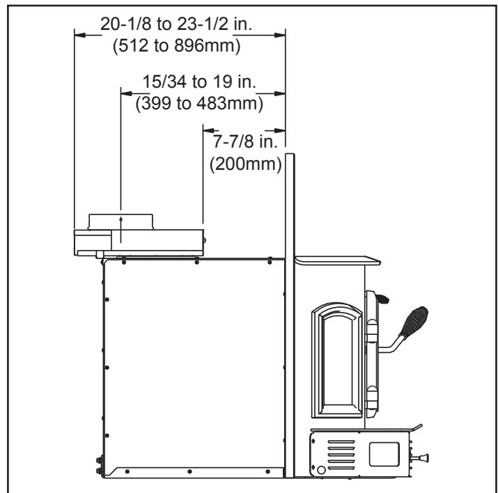
Figure 7.4 - Side View With Optional Offset Adapter
