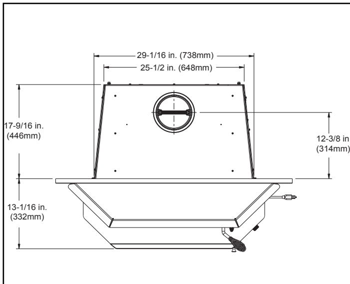
Figure 7.1 Top View
