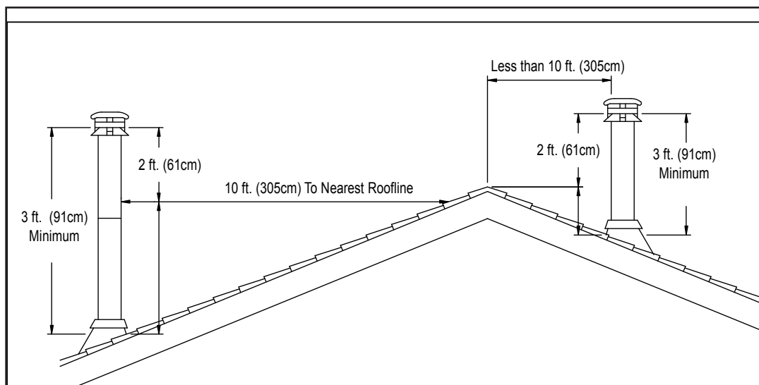
Figure 10.1 Pitched Roof
