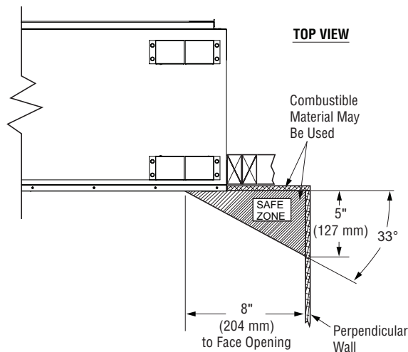
Figure 5 - Clearances for Combustible Mantels
