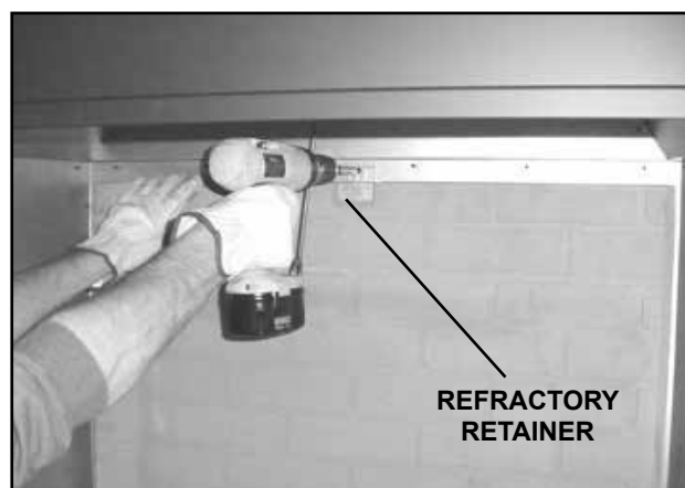
Figure 8.4 Attach Back Refractory
