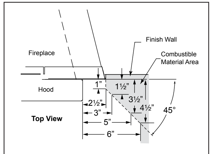
Figure 6.4 Mantel Leg Clearance
