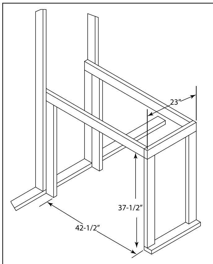
Figure 4.3 Framing Specifications
