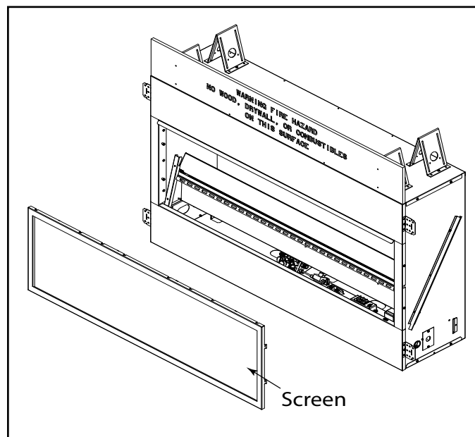
Figure 5.6 - Gas and Electrical Access - Remove Screen
