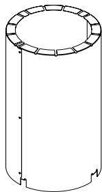
Assembled Diameter: 14 1/2 in./368 mm Height: 24 in./610 mm AS8 Straight Attic Insulation Shield
