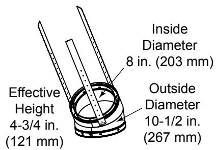
SL315/SL330 Offset/Return
