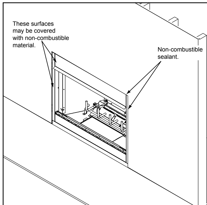
Figure 7.1 Non-combustible Facing
