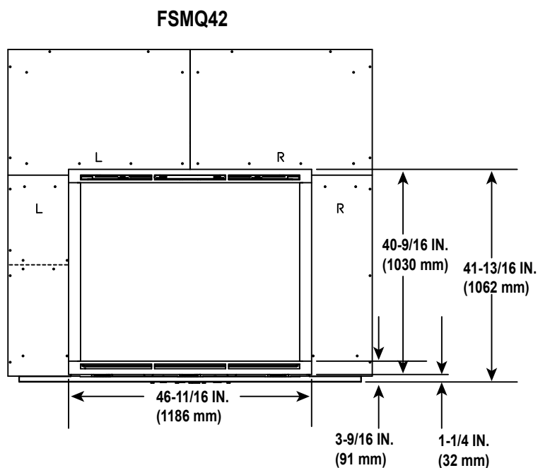
Figure 3.3 Decorative Barrier Front Dimensions
