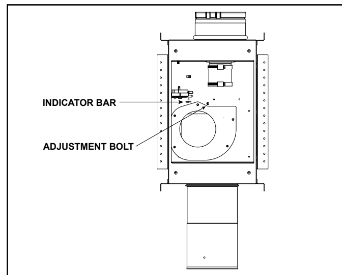
Figure 4.17 Baffle Adjustment Location - PVI-SLP-B
