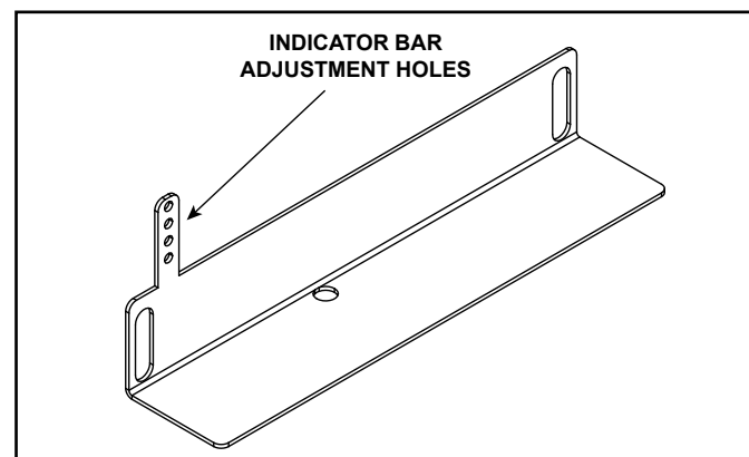
Figure 4.18 Baffle Adjustment - PVI-SLP-B
