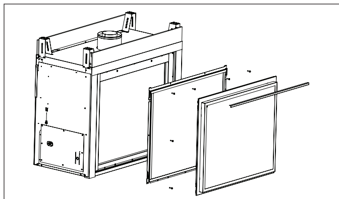
Figure 4.2 Exterior Glass Cleaning
