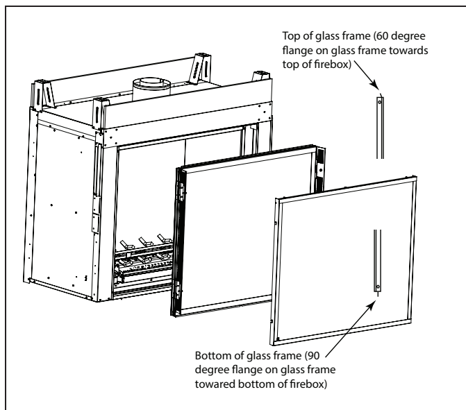
► Figure 4.1 Interior Glass Cleaning
