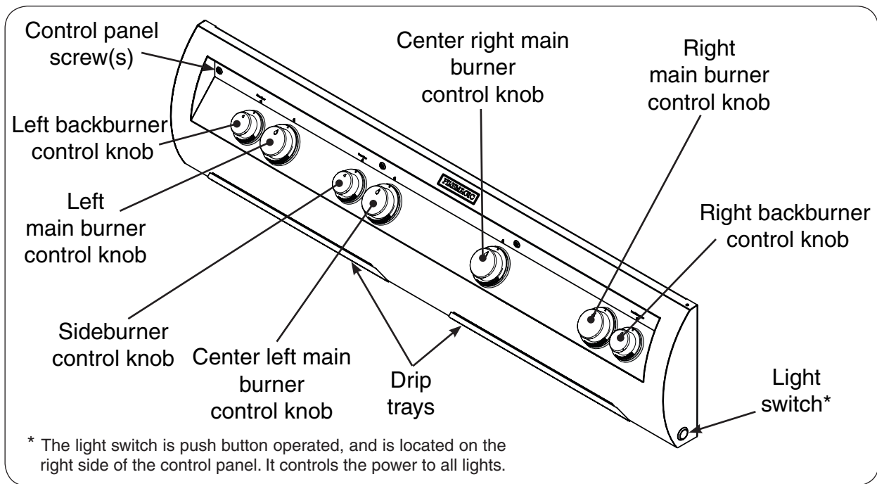
Fig. 24-1 E1060s controls
