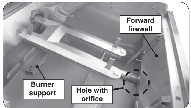
Fig. 39-2 Remove burners
