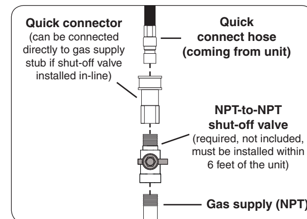
Fig. 20-5 Connecting to a gas line
