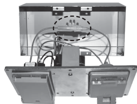
Fig. 37-4 Carefully open box and replace fuse (red wire)
