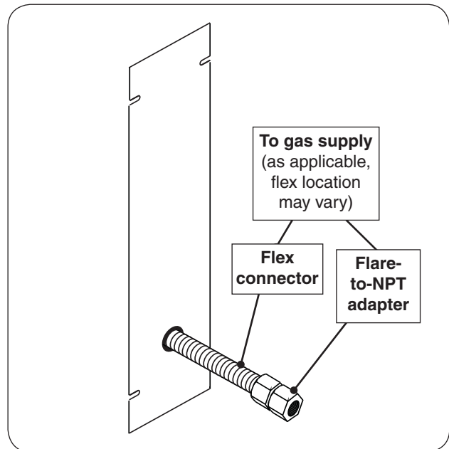
Fig. 16-1 Connect gas and secure plate
