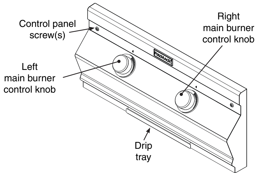
Fig. 22-1 C430s controls
