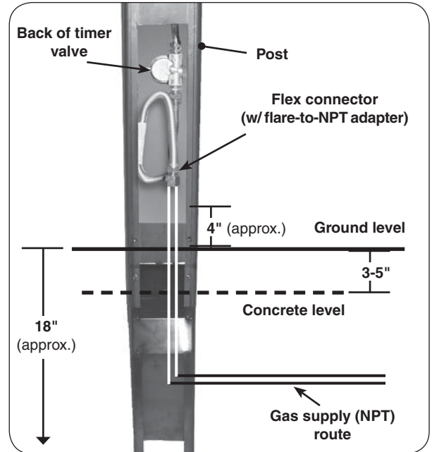
Fig. 17-1 In-ground install orientation
