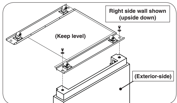
Fig. 1-2 Install right wheel assembly to bottom of right side wall
