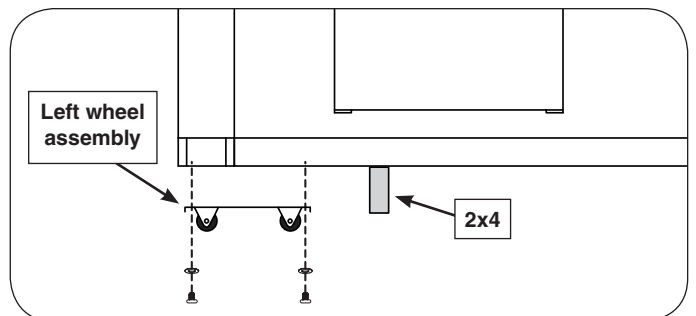
Fig. 2-3 Install left wheel assembly
