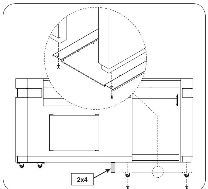
Fig. 2-4 Install right wheel assembly
