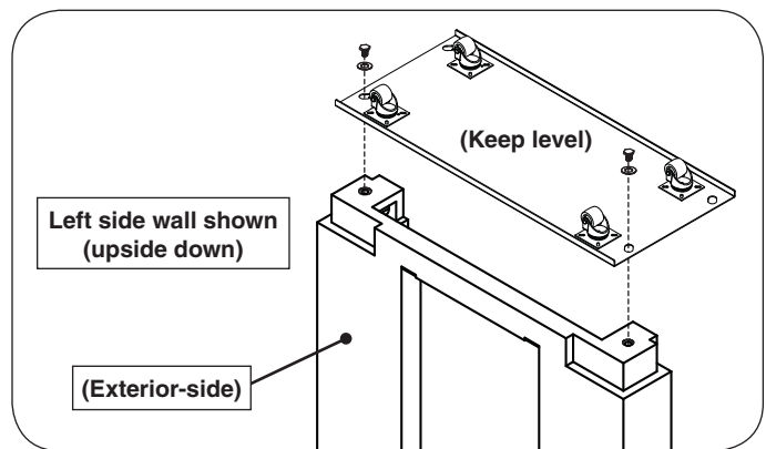
Fig. 1-1 Install left wheel assembly to bottom of left side wall
