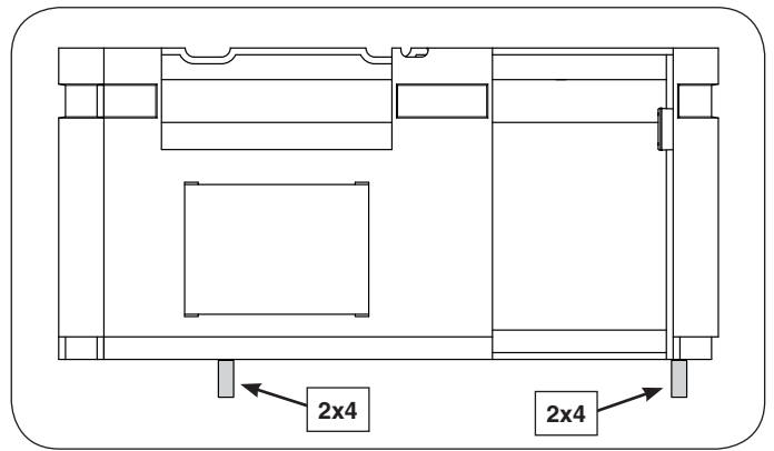
Fig. 2-1 Place 2x4's under island enclosure
