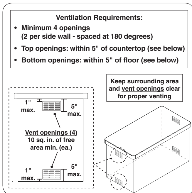
Fig. 11-1 Ventilation detail
