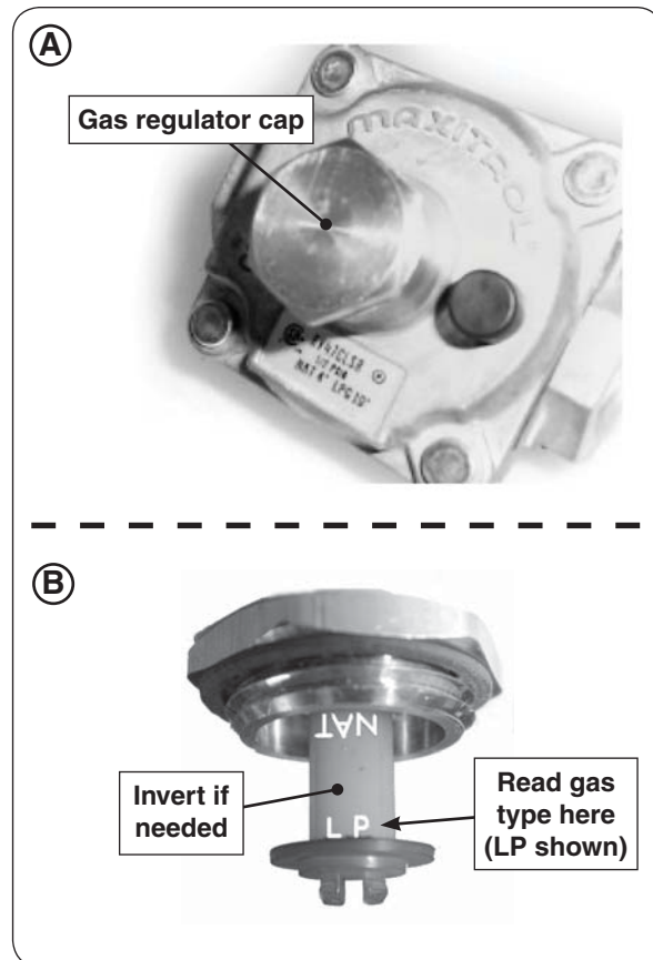
Fig. 23-1 Convert regulator
