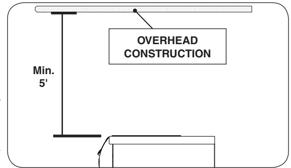
Fig. 9-1 Overhead requirements
