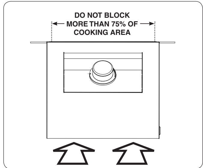
Fig. 10-1 Ventilation Diagram
