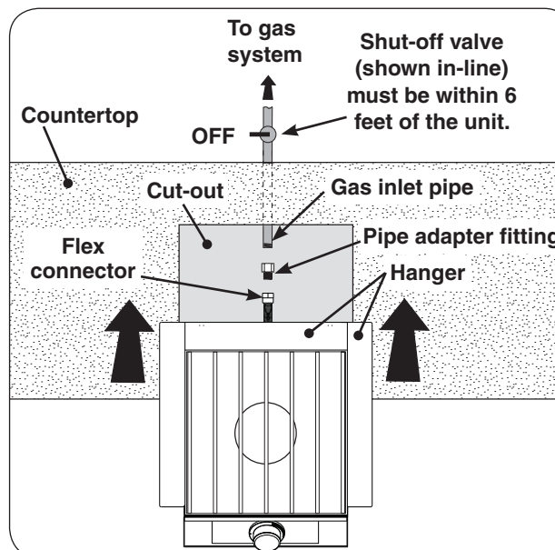
Fig. 15-4 Household propane & natural gas diagram
