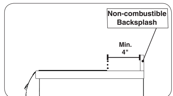
Fig. 9-5 Backsplash clearance
