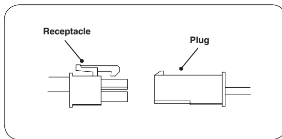
Fig. 16-1 Connection detail
