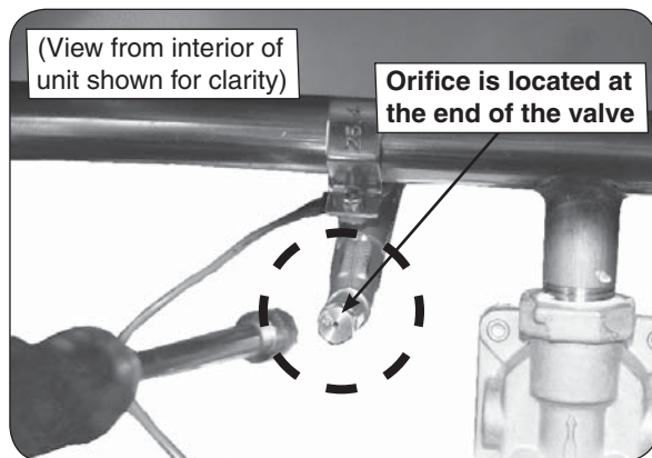
Fig. 24-3 Orifice location
