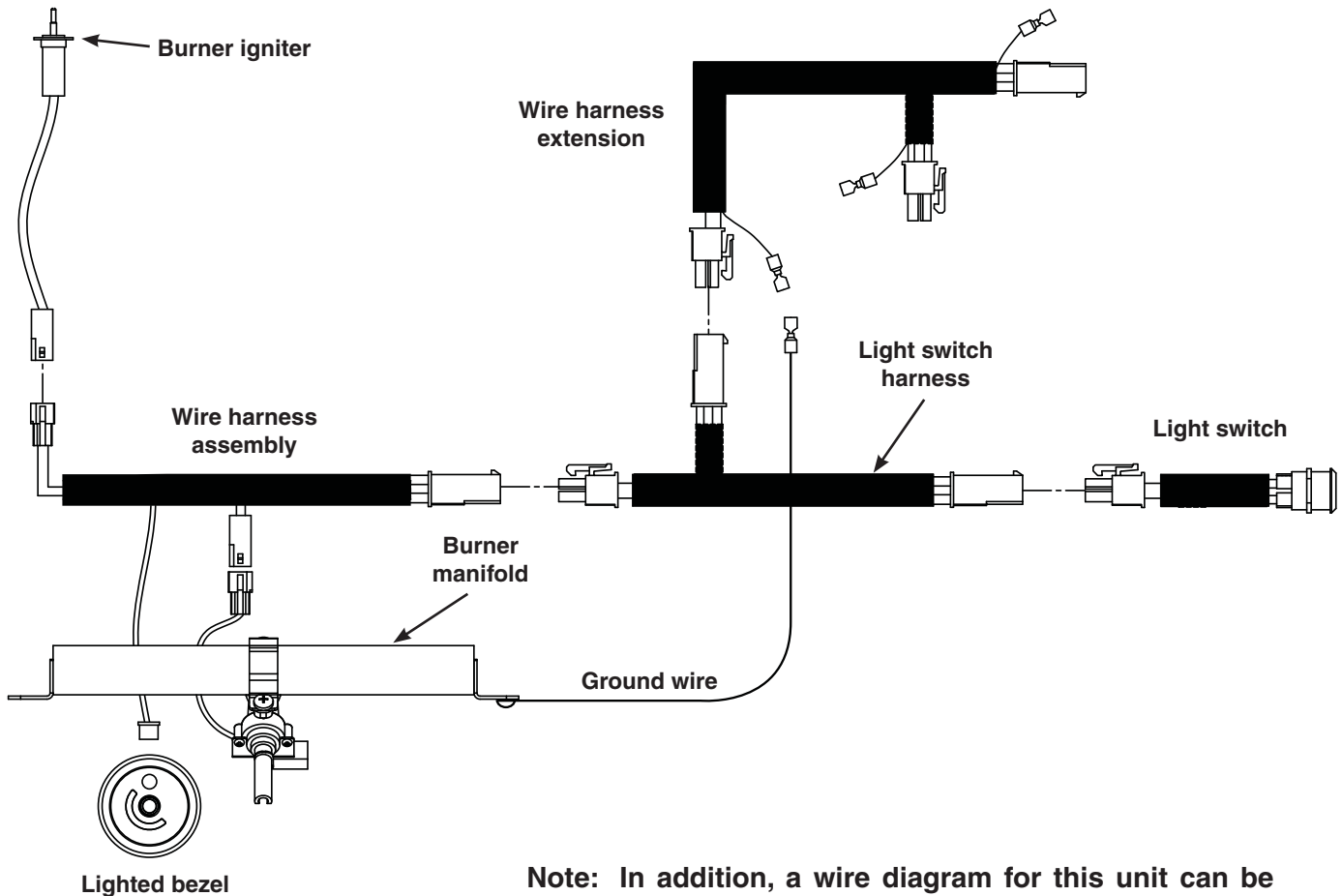
SIDEBURNER WIRING DIAGRAM
