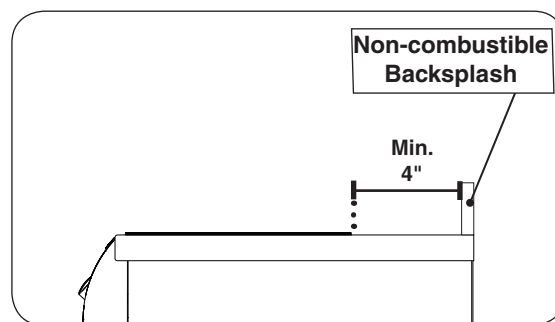
Fig. 10-4 Backsplash clearance
