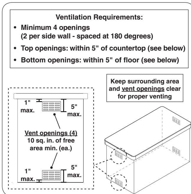
Fig. 12-1 Ventilation detail
