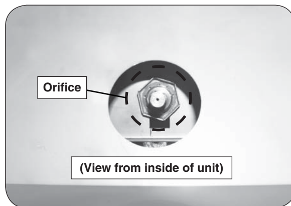
Fig. 26-2 Orifice location
