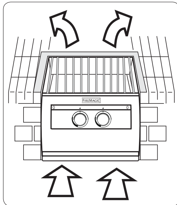
Fig. 11-1 Ventilation Diagram
