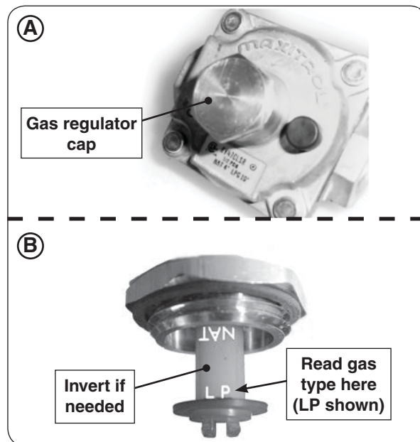
Fig. 33-1 Regulator conversion
