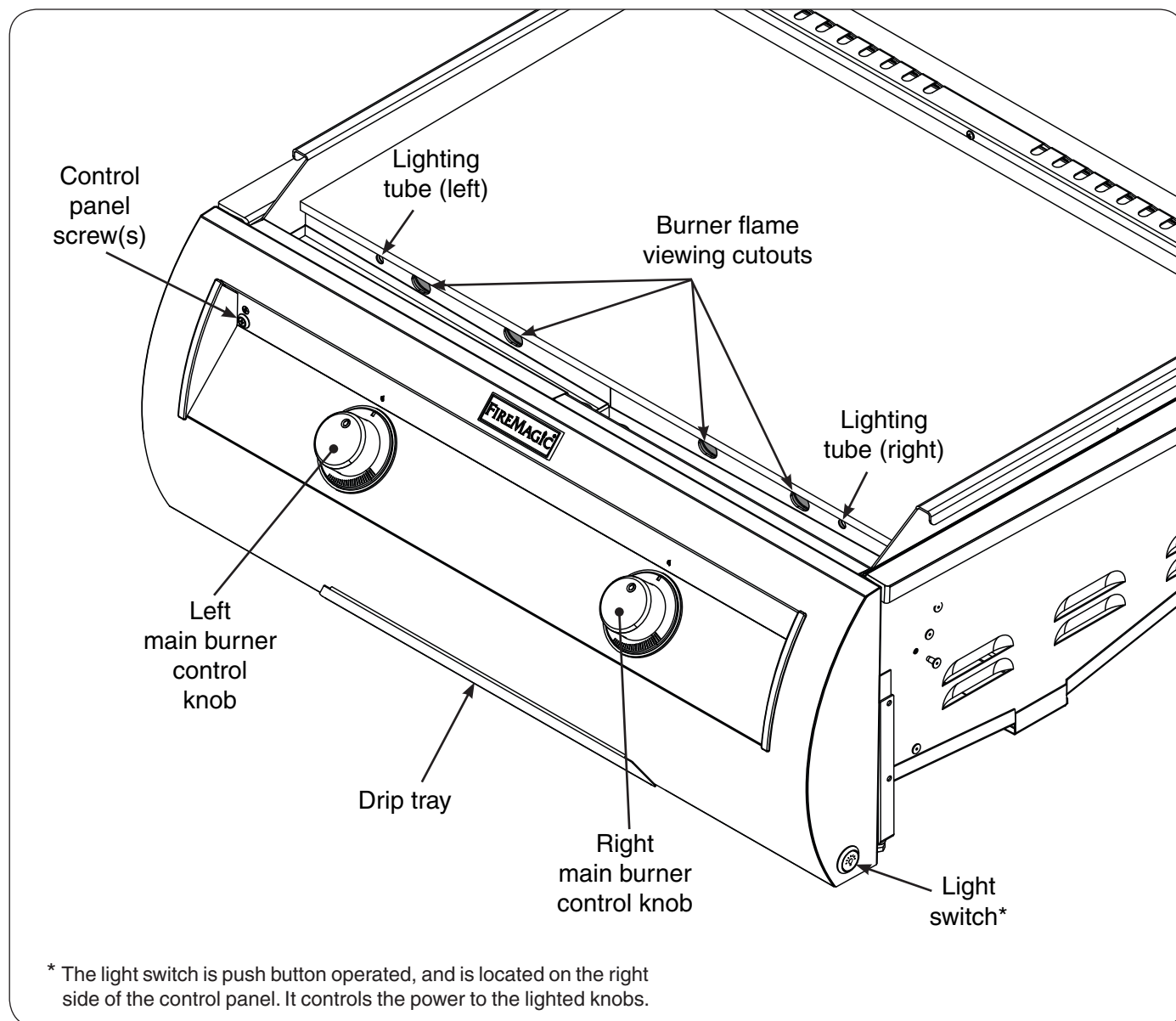
Fig. 25-1 E660i Griddle controls
