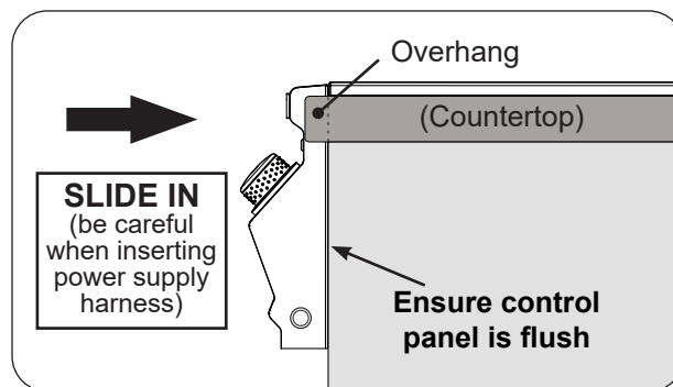
Fig. 26-1 Slide in unit (ensure flush)
