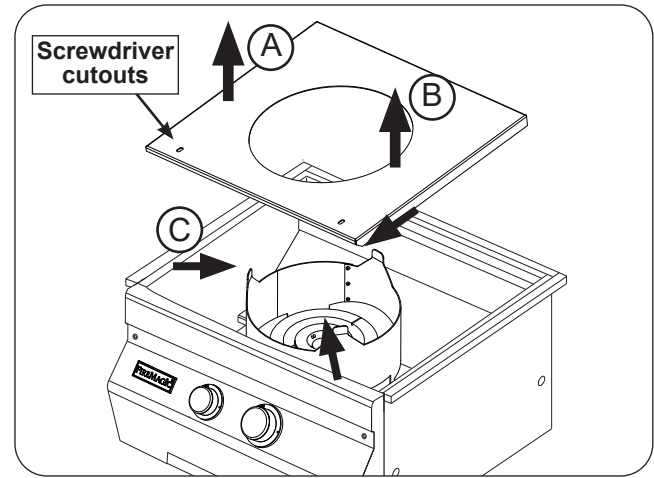
Fig. 39-1 Interior protection plate removal
