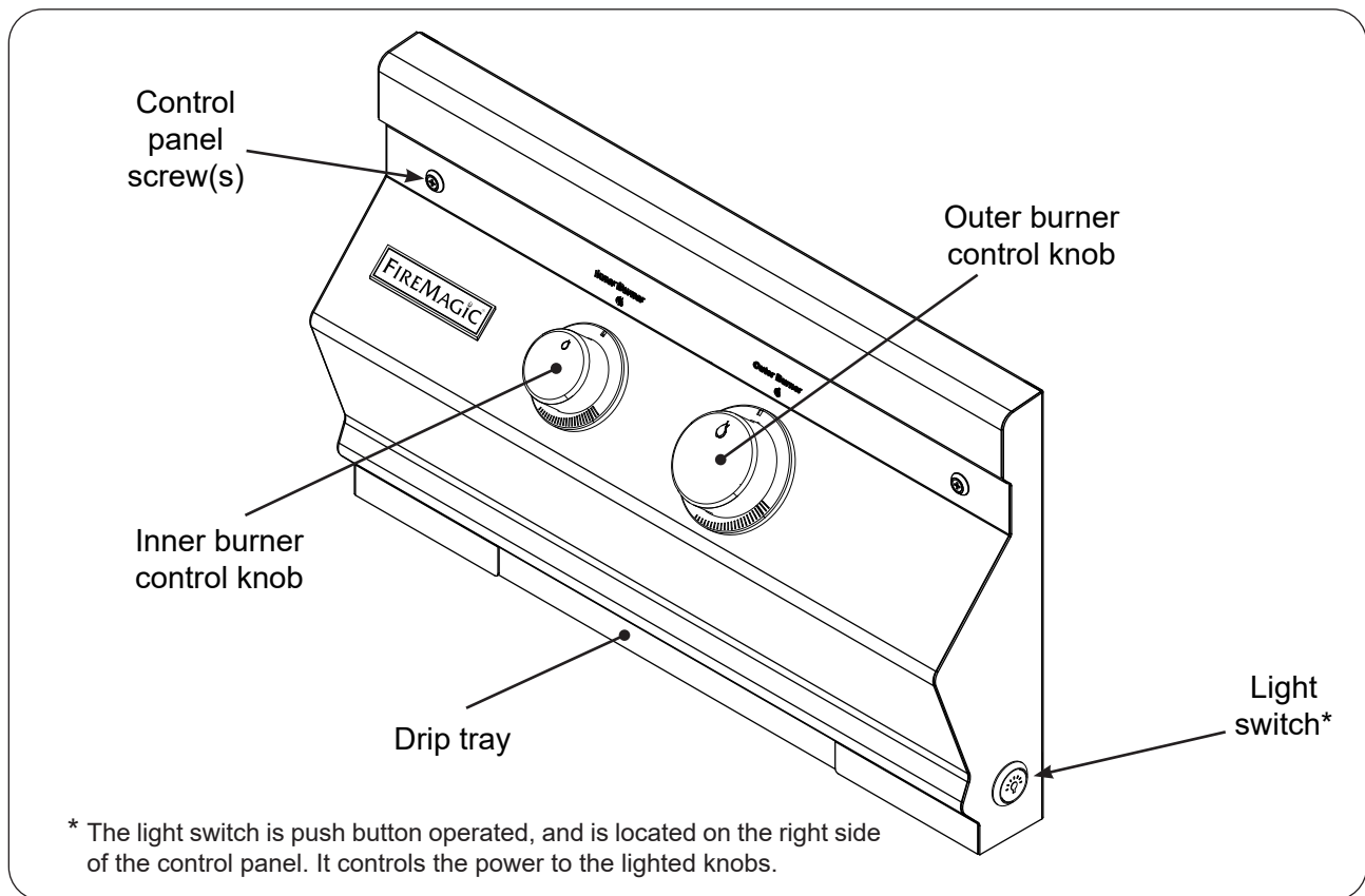
Fig. 32-1 Power burner controls
