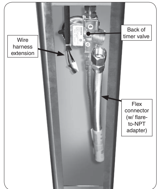
Fig. 17-2 Post interior detail
