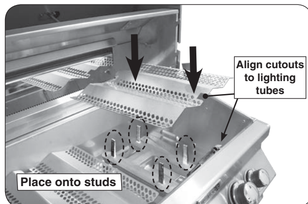
Fig. 22-1 Install flavor grids
