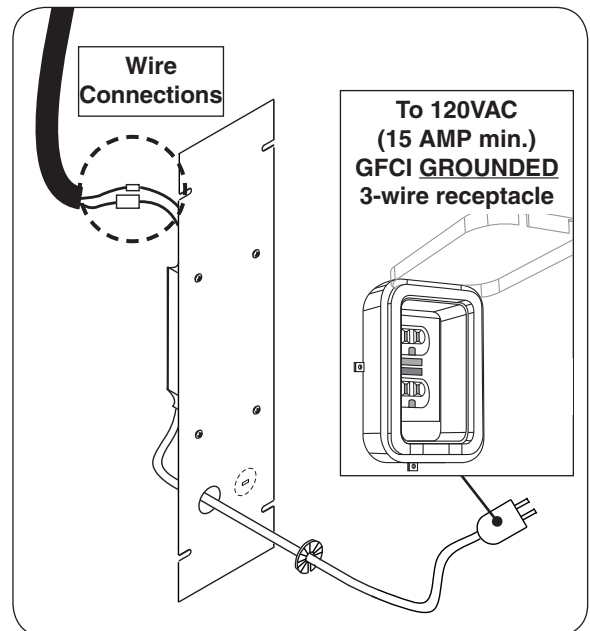
Fig. 21-2 Connect: Wires, Plate, Power
