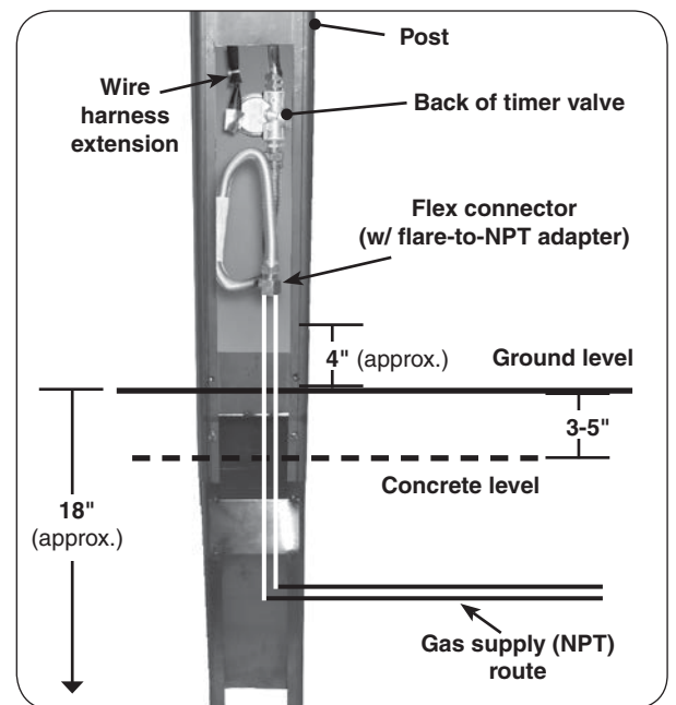
Fig. 19-2 In-ground install orientation
