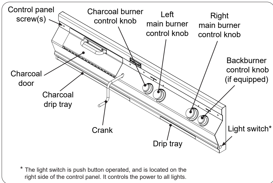
Fig. 35-1 A830 controls
