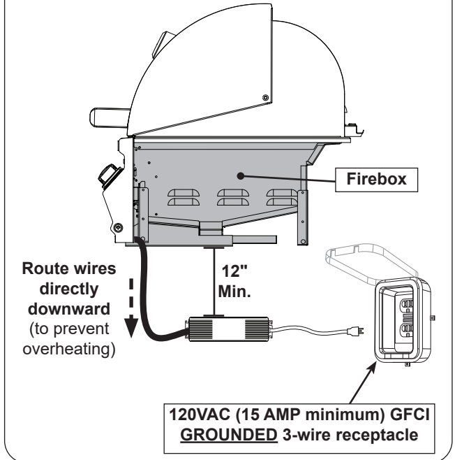
Fig. 29-1 Electrical installation
