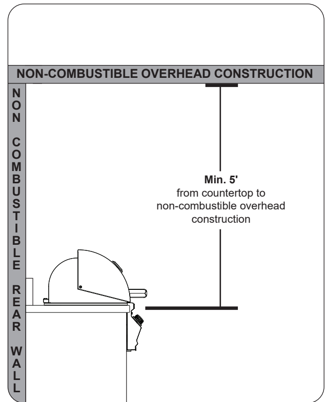
Fig. 17-1 Overhead requirements
