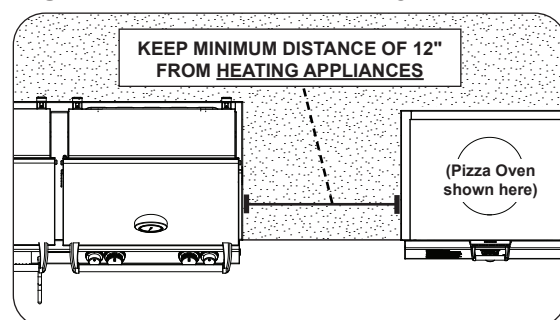
Fig. 19-4 Clearance to heating appliances
