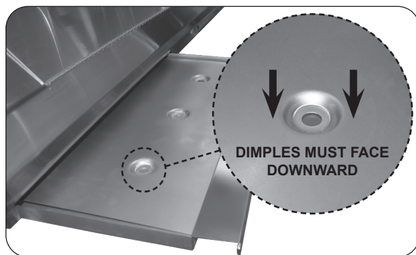
Fig. 34-4 Charcoal drip tray heatshield placement
