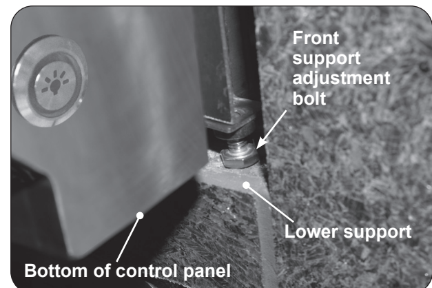
Fig. 28-4 Front support adjustment bolts
