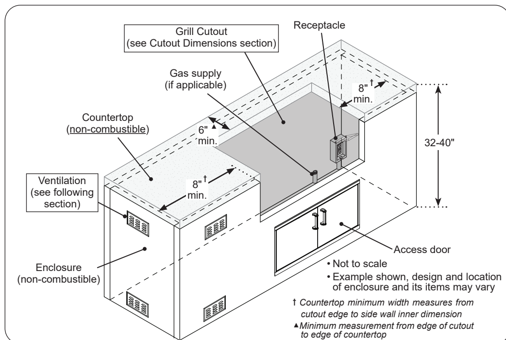
Fig. 11-1 Enclosure specifications
