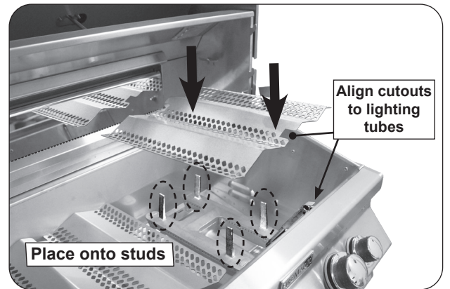
Fig. 31-2 Install flavor grids
