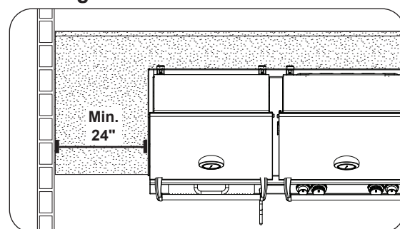
Fig. 19-2 Side wall clearance
