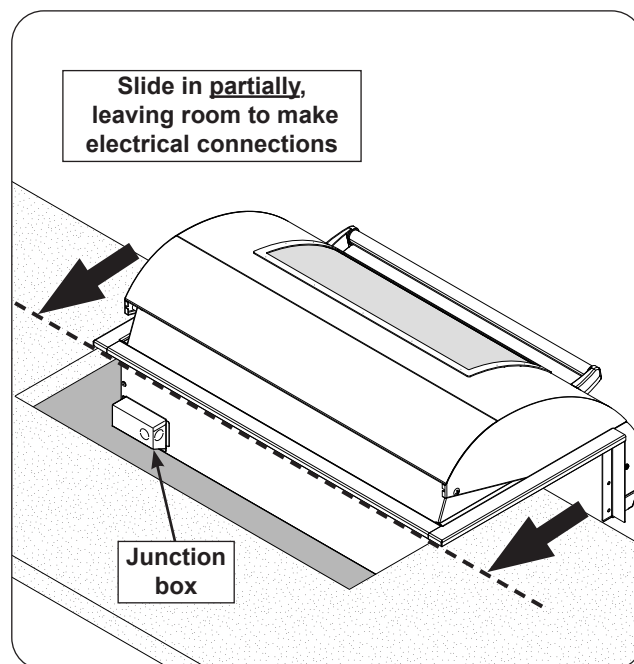
Fig. 26-2 Position unit for wiring
