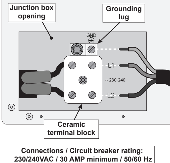
Fig. 27-2 Wire connection diagram
