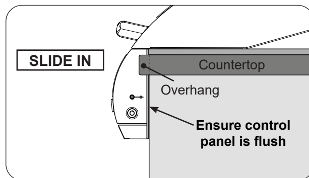
Fig. 27-3 Slide in unit (ensure flush)
