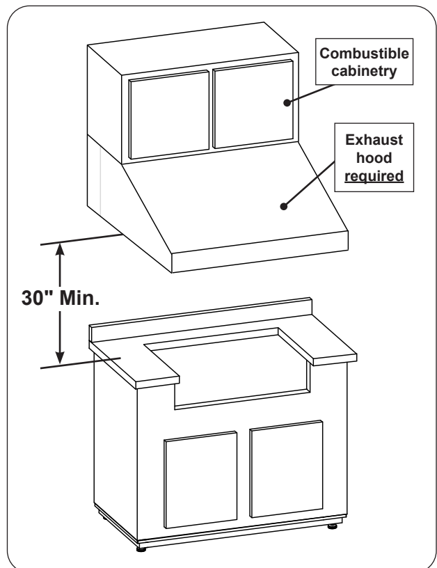
Fig. 16-2 Overhead cabinetry requirements
