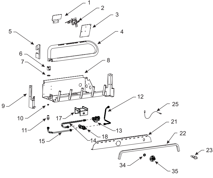
24" BURNER
