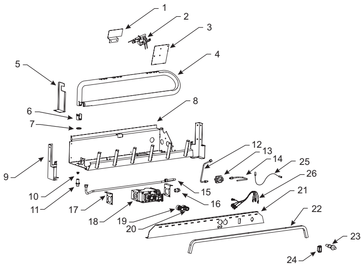
30" BURNER
