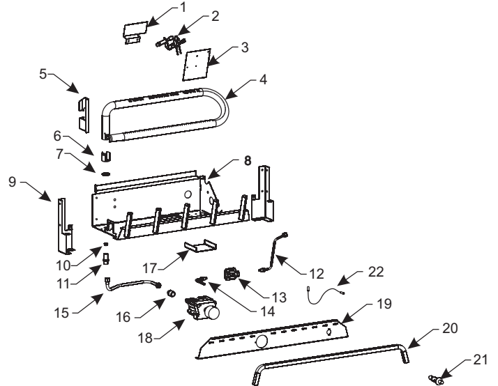
24" BURNER
