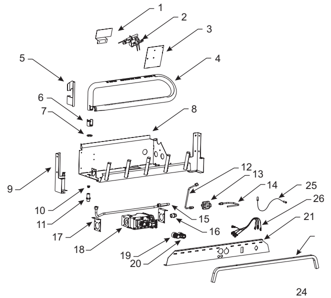
24" BURNER
