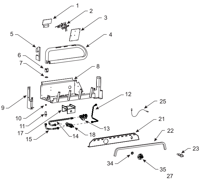
18" BURNER
