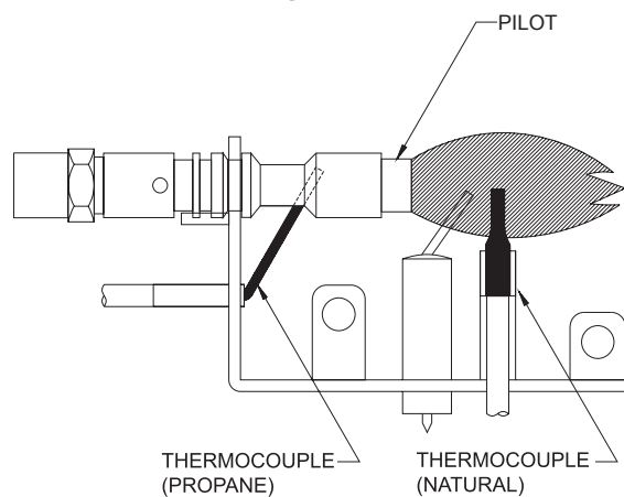
Correct Pilot Flame Pattern for VFDT & VFDM Figure 20
