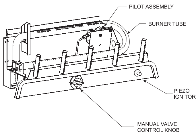
Manual Valve for VFDM Series Figure 17
