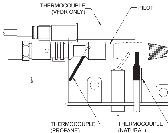
Incorrect Pilot Flame Pattern for VFDR Figure 21
