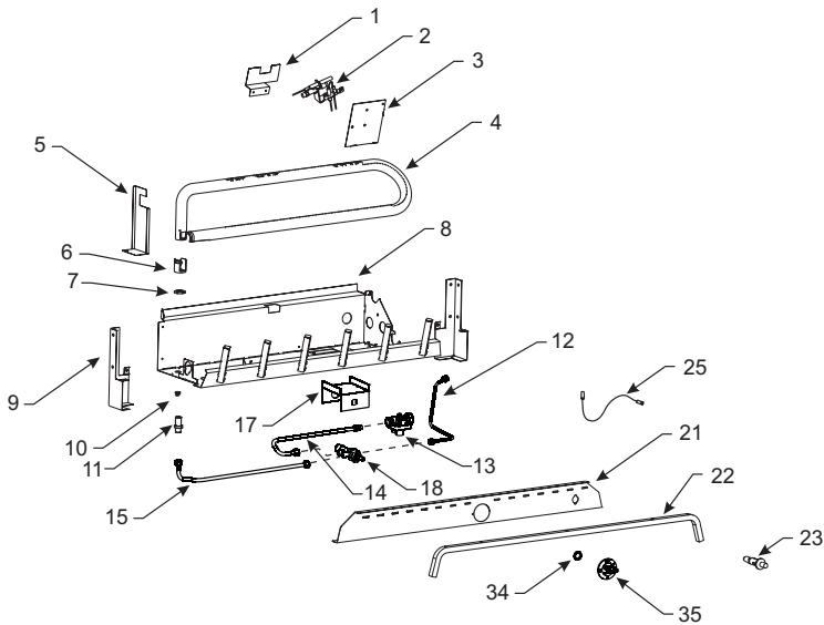
30" BURNER
