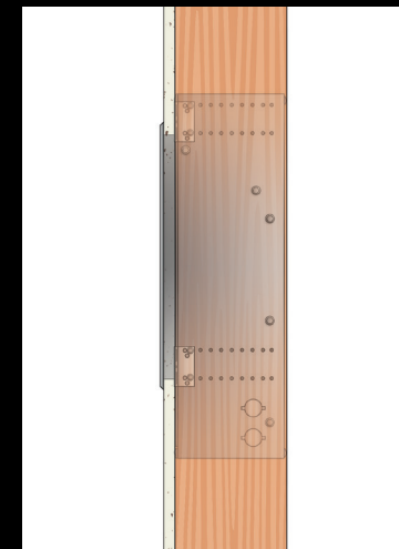
Recessed Installation shown in 2x6 stud walls
