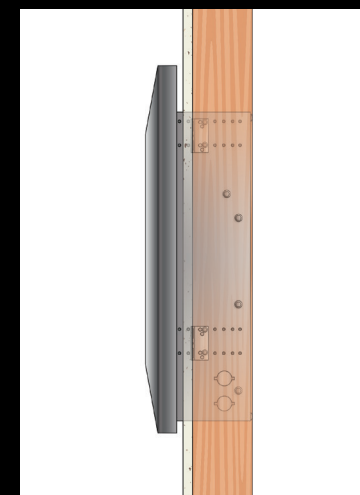
Partially Recessed Installation shown in 2x4 stud walls
