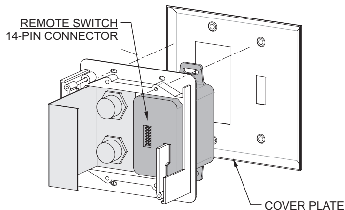
Figure 74 - Proflame Receiver Body Back
