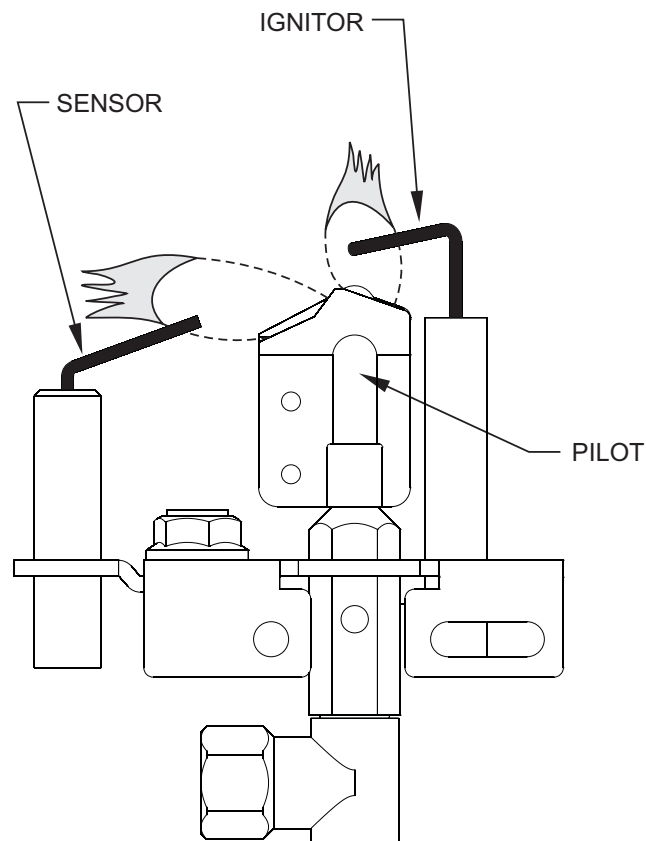
Figure 70 - Incorrect Pilot Flame Pattern
