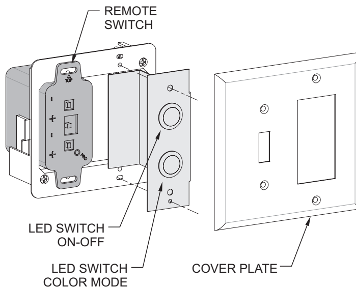
Figure 73 - Proflame Receiver Body Front
