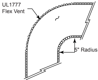
Figure 17 Minimum Radius for Flex Vent Section
