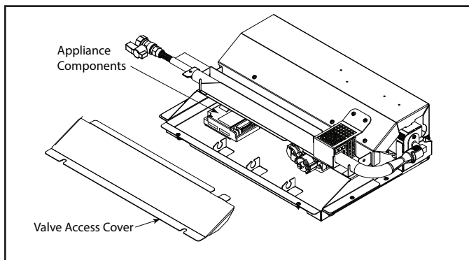
Figure 6.1 Burner Assembly
