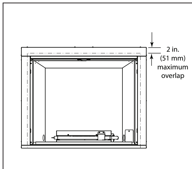
Figure 3.5 Membrane Overlap
