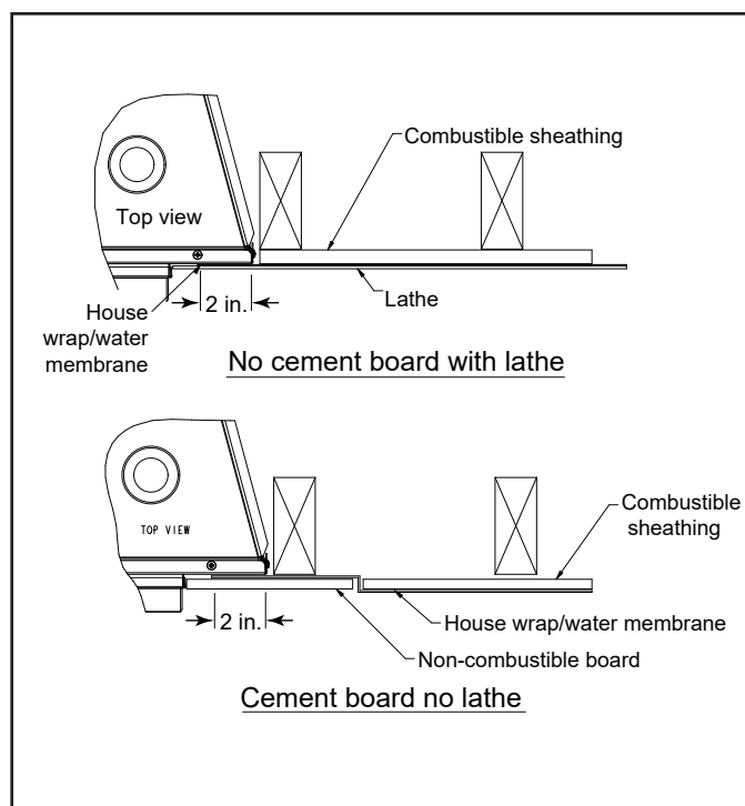
Figure 3.6 Moisture Membrane
