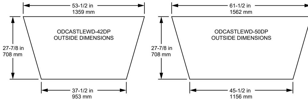
Figure 3. Drain pan dimensions
