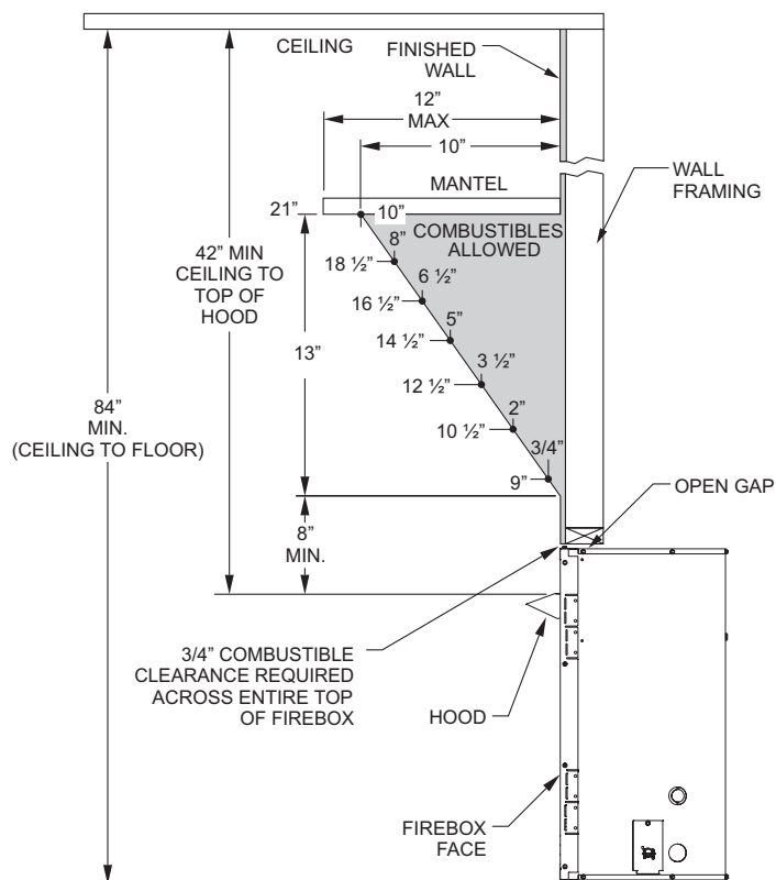
Figure 3 - Clearances to Combustibles (Based on 40,000 btu/hr burner system)
