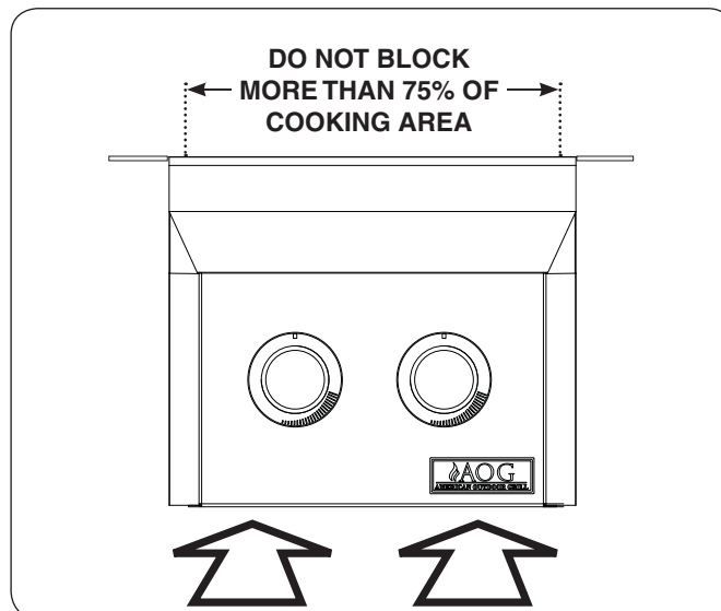
Fig. 10-1 Ventilation Diagram
