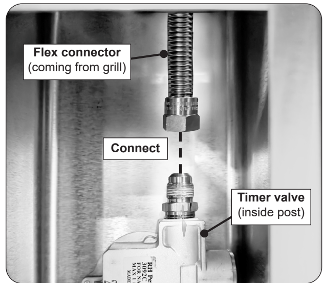
Fig. 20-1 Connect grill to timer
