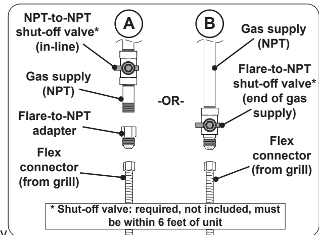
Fig. 20-3 Connecting to a gas line
