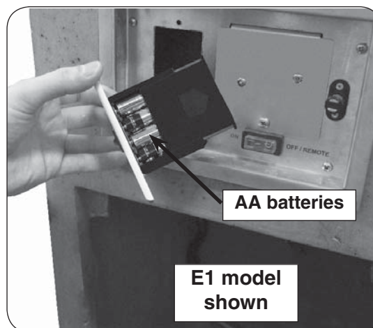
Fig. 36-3 Remote receiver batteries
