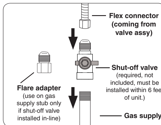
Fig. 20-3 Connecting to a gas line
