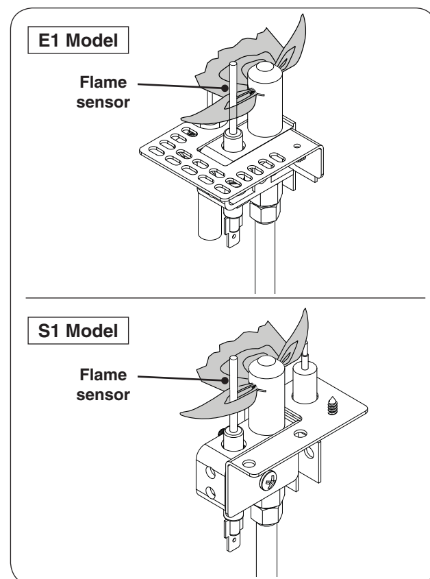
Fig. 31-2 Proper pilot flame
