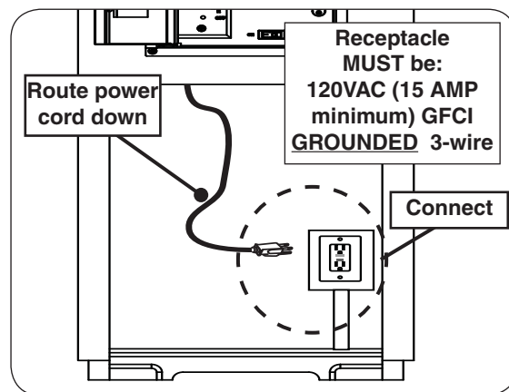
Fig. 21-1 Route and connect power supply cord
