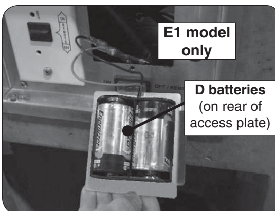
Fig. 36-4 Burner system batteries
