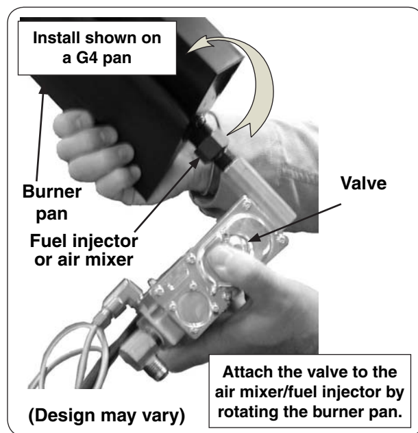
Fig. 5-2 Install valve
