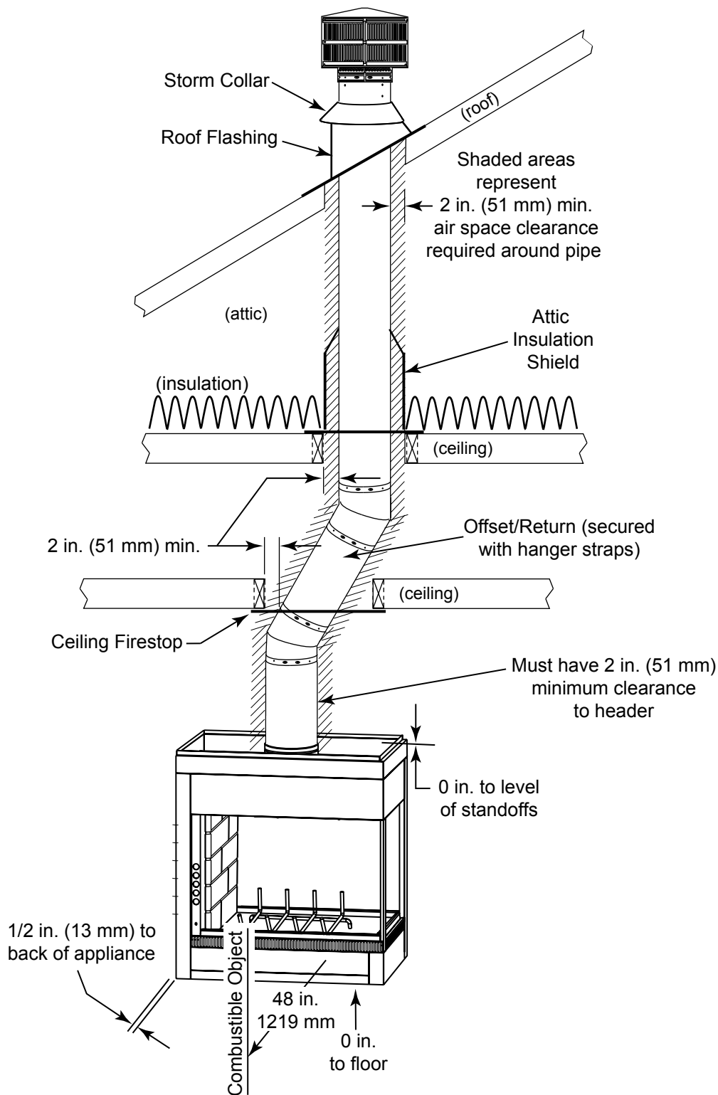
Figure 6.2 Air Space Clearances
