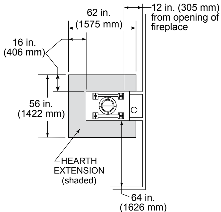
Figure 6.1 Fireplace Locations
