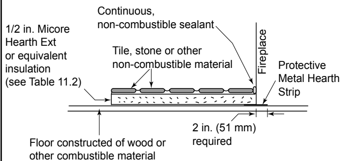
Figure 11.1 Hearth Extension Dimensions
