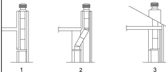
Figure 9.2 Chase Constructions
