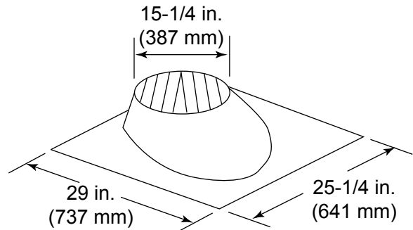
RF570 Roof Flashing 15-1/4 in. (387 mm)
