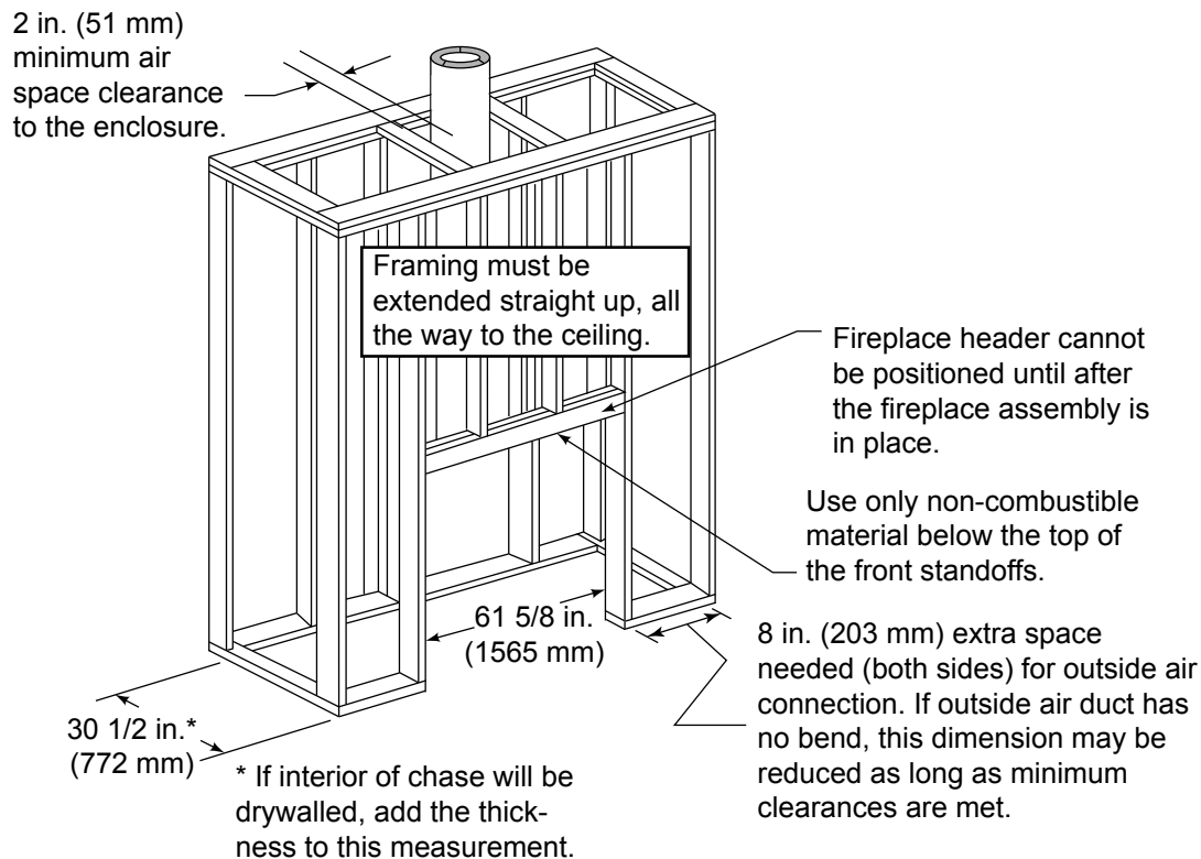
Figure 6.4 Framing the Fireplace
