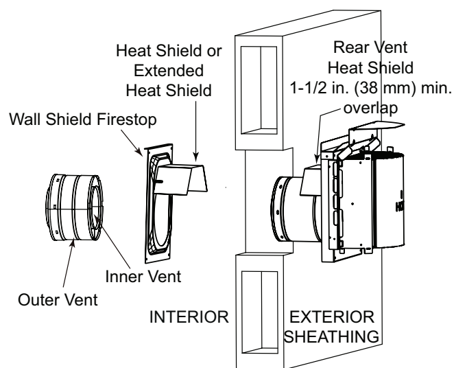
Figure 3.1 Venting through the Wall
