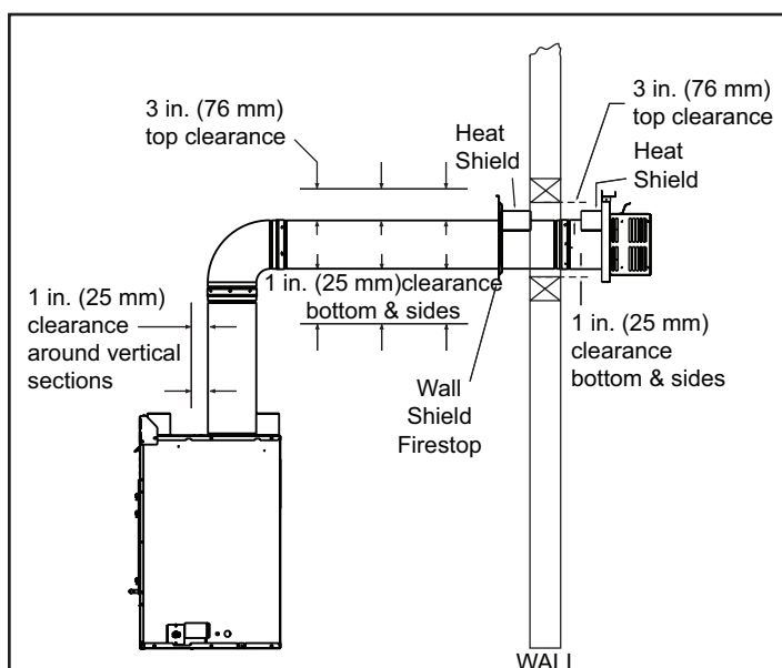
Figure 2.1 Horizontal Venting Clearances to Combustible Materials - Top Vent
