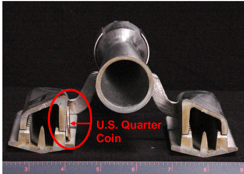
Upside down "E" burner cut in half.
