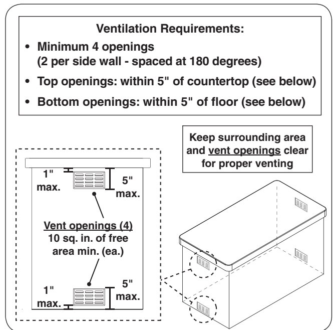
Fig. 11-1 Ventilation detail
