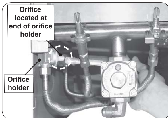
Fig. 21-3 Orifice location
