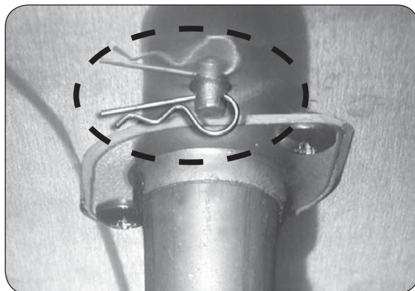
Fig. 21-1 Remove burner clip
