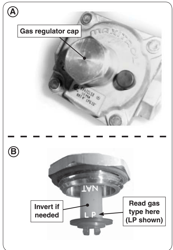
Fig. 20-1 Convert regulator
