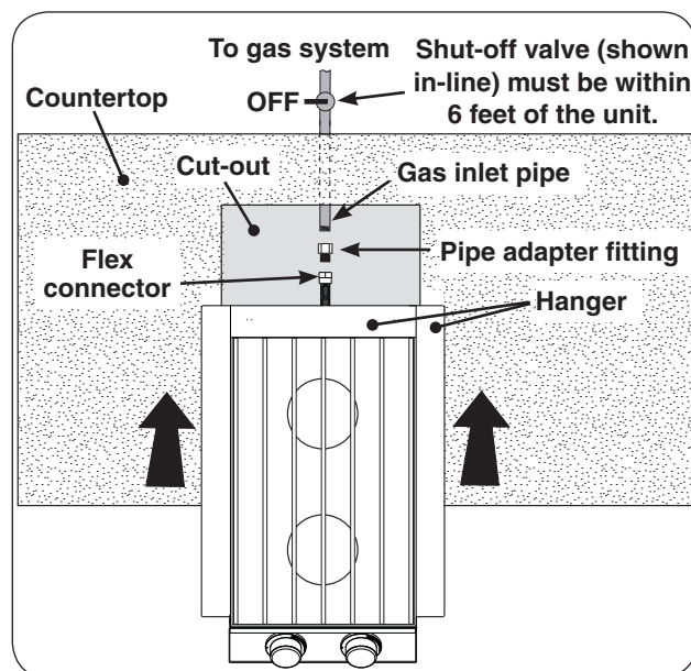
Fig. 15-4 Household propane & natural gas diagram
