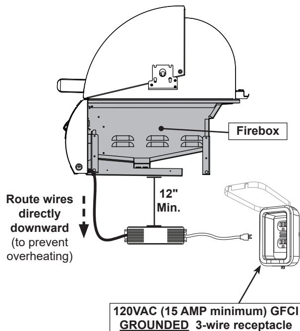
Fig. 29-3 Electrical installation
