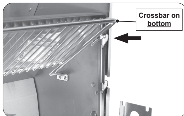
Fig. 33-3 Place warming rack in storage position
