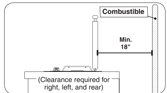
Fig. 7-4 Clearance 'C' Diagram
