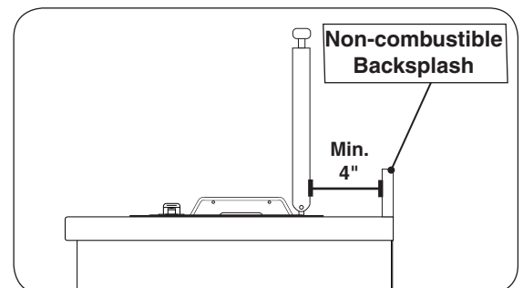
Fig. 7-5 Backsplash clearance
