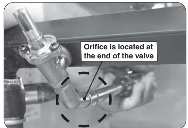
Fig. 21-3 Orifice location
