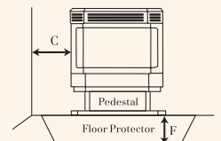
Front View - Free-Standing
