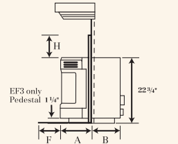
Side View - Insert
