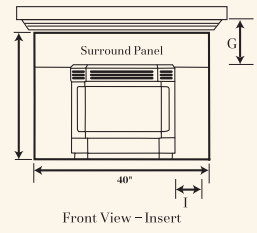
Front View - Insert
