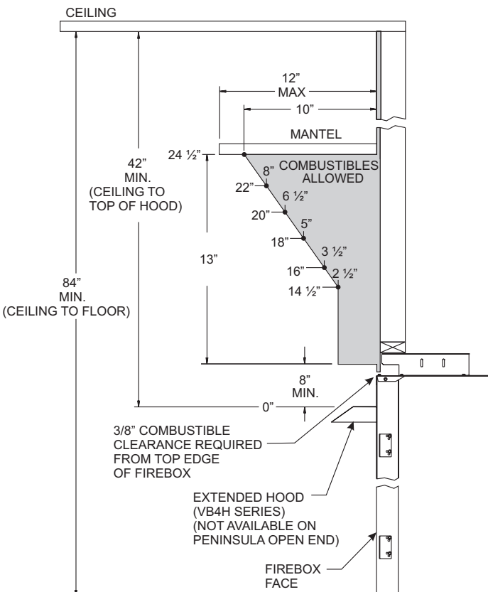
Figure 3b - Mantel Clearances with Optional Extended Hood
