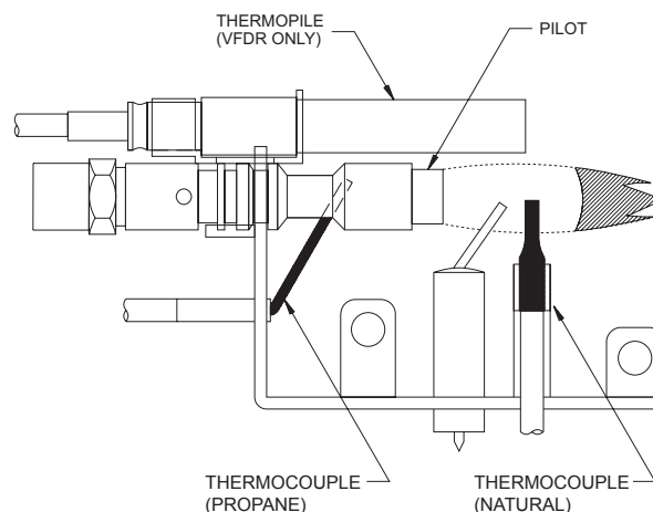
Incorrect Pilot Flame Pattern for VFDR Figure 22
