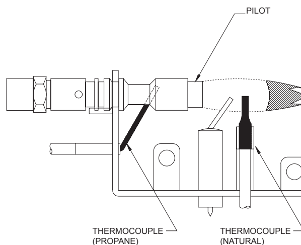
Incorrect Flame Pattern for VFDT & VFDM Figure 23
