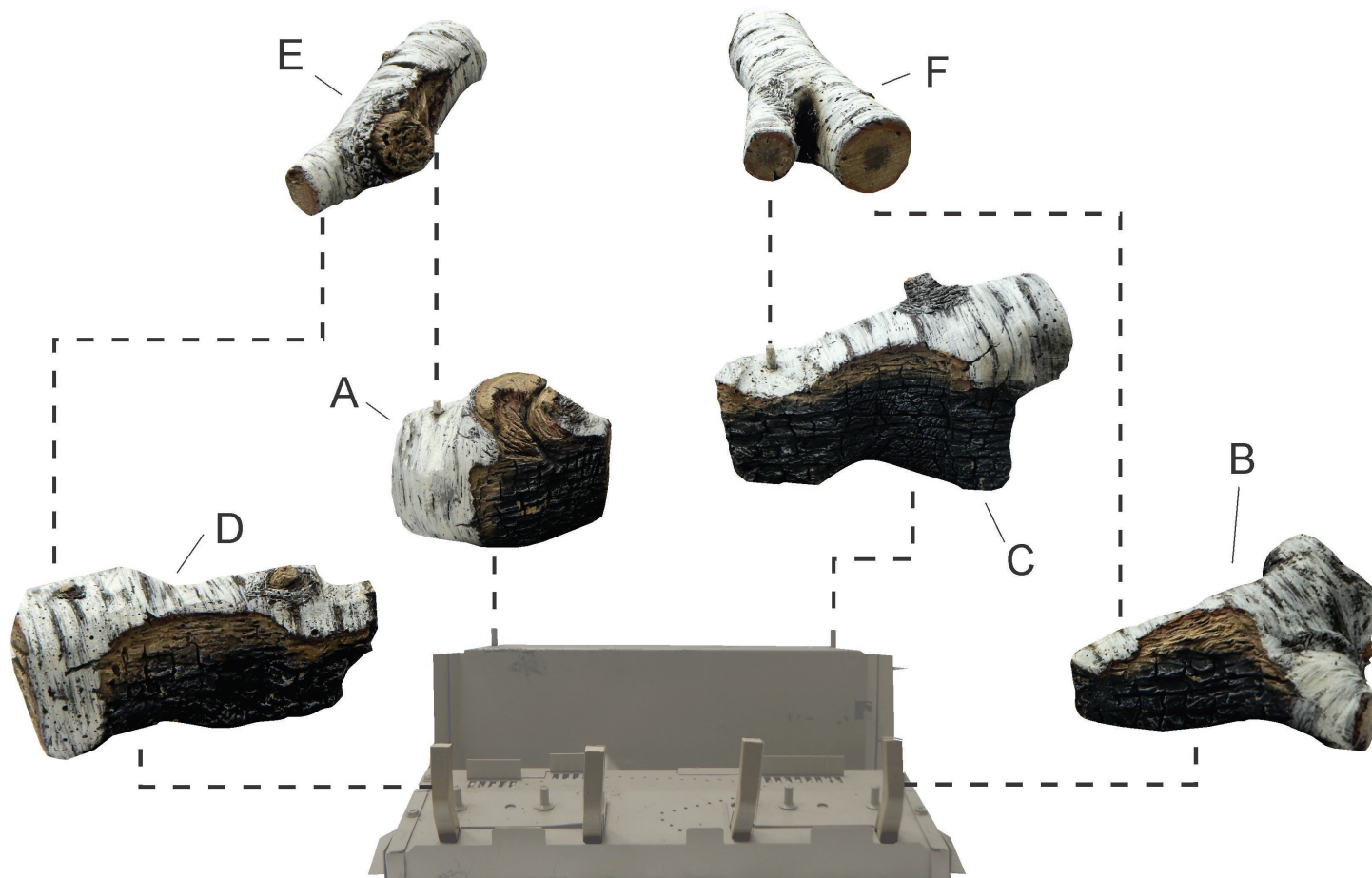
LS18CB - Figure 1
